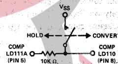
"Hold" Circuit Figure 7
